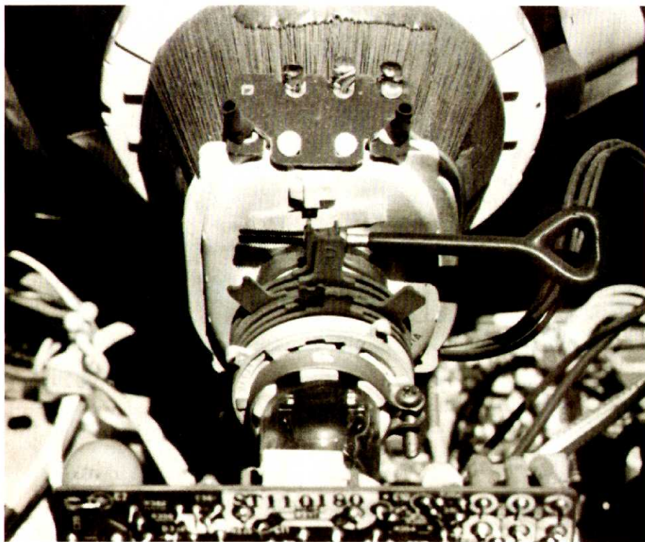
Figure 1. This rear view of a typical 19" color TV set shows the yoke coil (held in place by a large turn key) and color purity and convergence controls on the neck of the picture tube.
