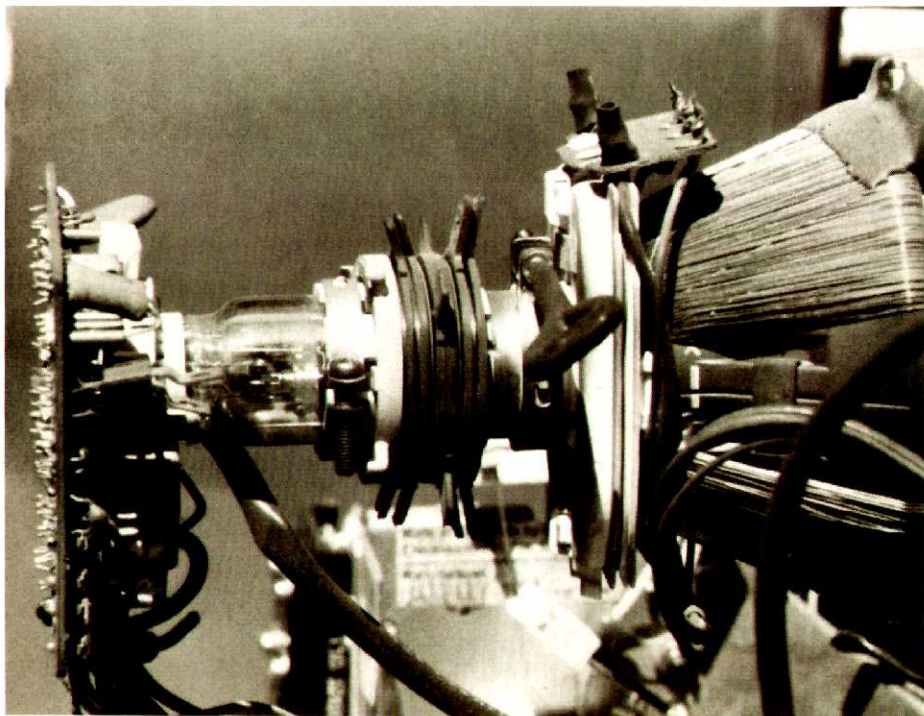
Figure 2. A side view of the purity and convergence tabs on the picture tube.
