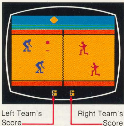
Figure 4—Score Display
